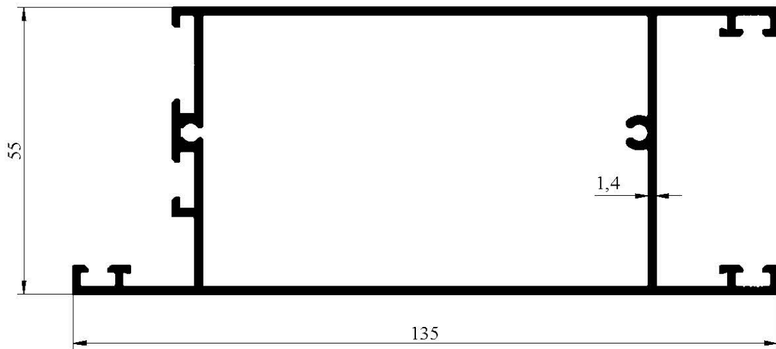
1157 1,593 kg/m
