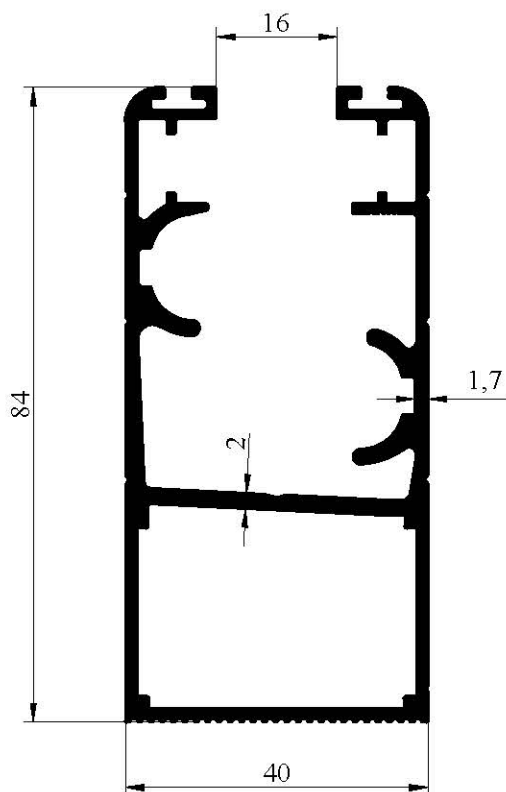
1184 1,520 kg/m
