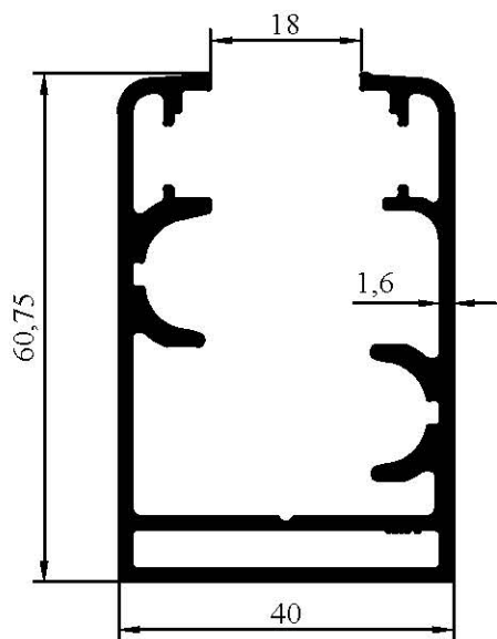
1147 1,260 kg/m
