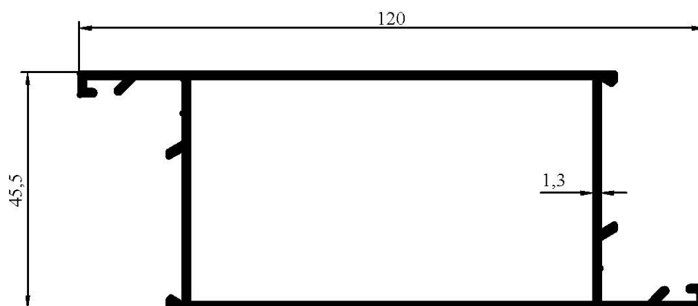
7000 1,130 kg/m
