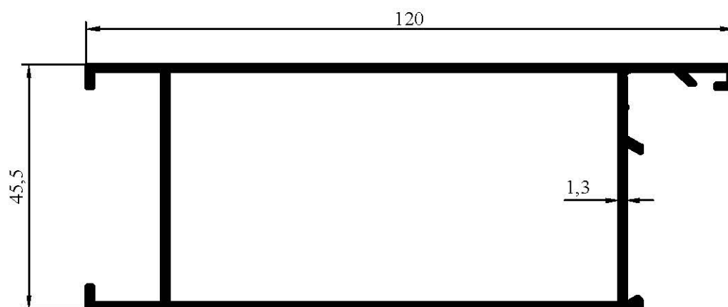
7001 1,160 kg/m
