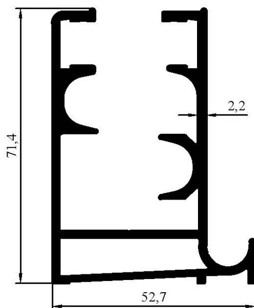
7075 1,640 kg/m
